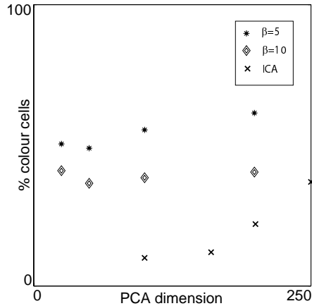
Fig. 3. Percentage of colour cells (mean saturation > 0.2 ) vs. PCA dimension for two values of \beta compared to ICA results of reference [9].
