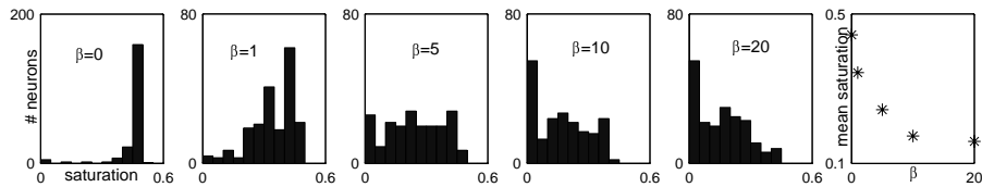
Fig. 2. Histograms of mean saturation for different values of \beta . Rightmost panel: mean of each histogram vs. \beta
