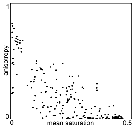
Fig. 4. Value anisotropy vs. mean saturation for a simulation of \beta = 5 .
